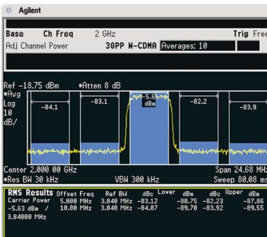
The PSA Series has excellent dynamic range for a W-CDMA adjacent channel power (ACP) measurement
