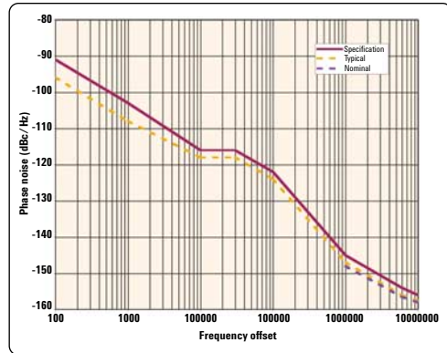
PSA Series phase noise performance plot (1 GHz center frequency)
