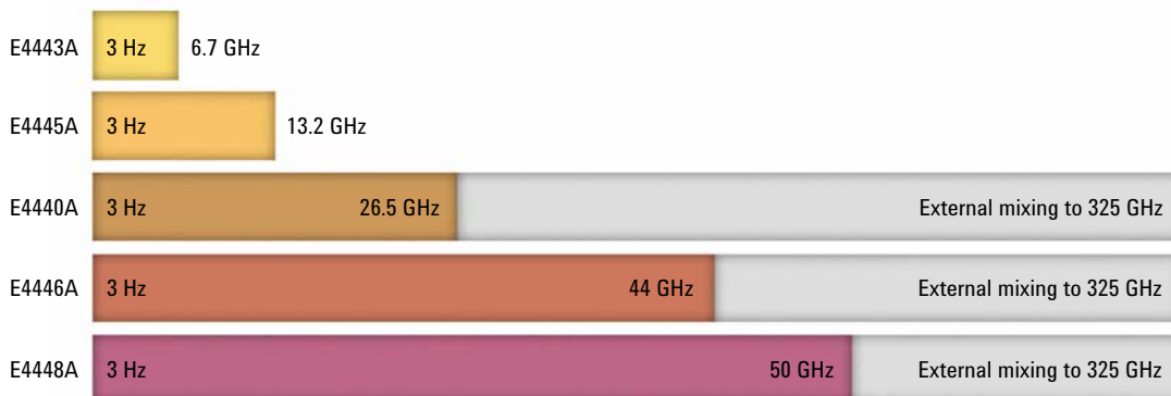
PSA Series frequency range summary
