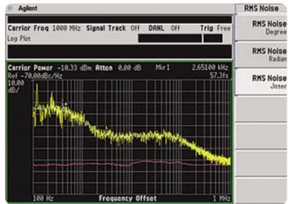
Log plot measurement
