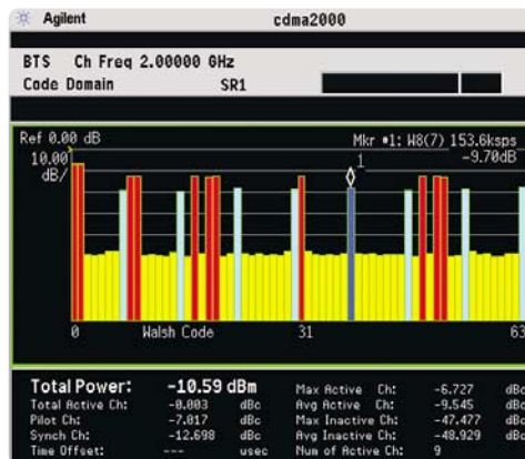
cdma2000 code domain analysis
