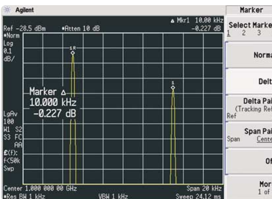
This figure illustrates 0.1 dB/division display resolution, 0.01 dB reference level resolution, and 0.001 marker resolution with averaging.
